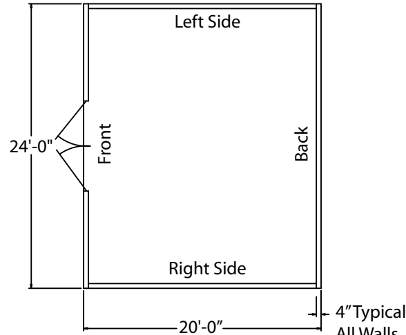
Floor Plan
